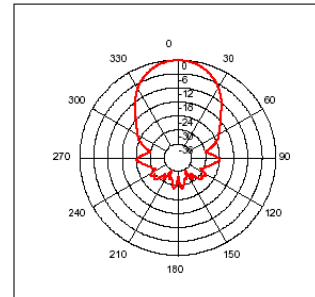
Fig. 2. Sonar radiation
