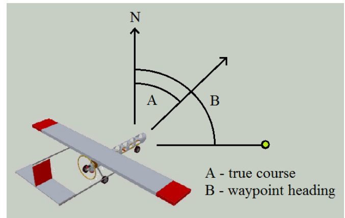
Fig. 3. Waypoint heading calculation
