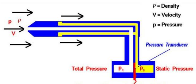
Fig. 3. Measurement principle
